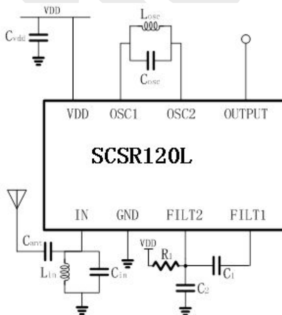
Fig.2. Typical Application Circuit (2)
