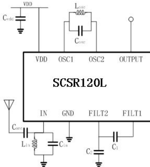
Fig.1. Typical Application Circuit (1)
